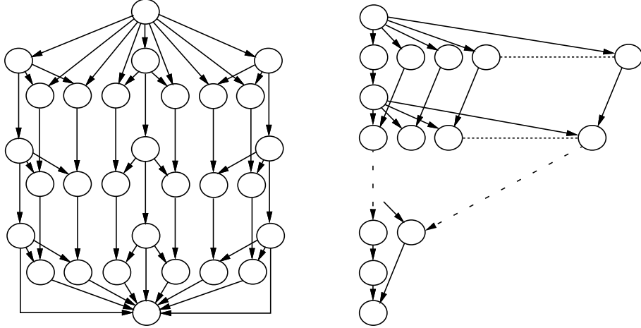
Figure 10: Task graphs for the block matrix multiplication (a) and the LU decomposition (b) algorithms.
