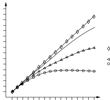
Figure 13: Speedup curves of the LU decomposition algorithm on a hypercube topology [44].
