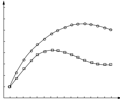
Figure 14: Speedup S(p) and efficacy \eta(p) for a odd-even transposition sort of 1024 elements [47].
